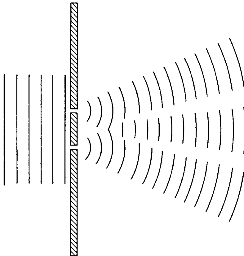
Fig. 8. Propagation of waves through two small holes.
