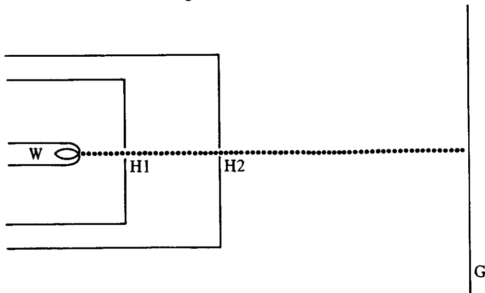
Fig. 1. Electron gun.
